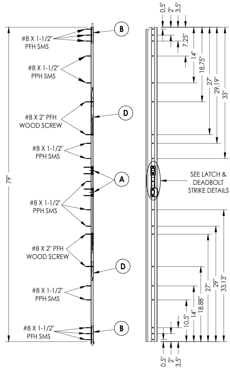
HURRICANE ASTRAGAL ASSEMBLY
