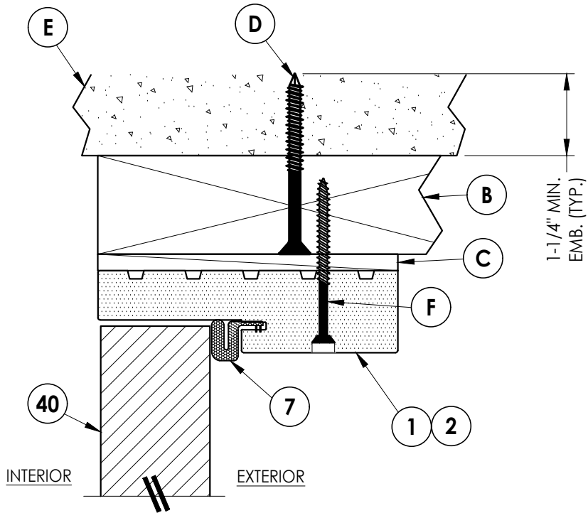
3 VERTICAL CROSS SECTION 5 Inswing Shown (Outswing Similar) 2X Buck Construction
