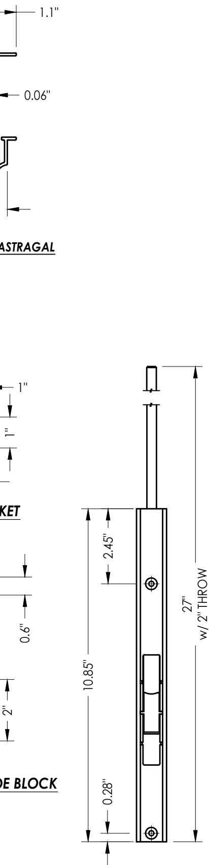
D SLIDE LOCK FLUSHBOLT ASSEMBLY HURRICANE ASTRAGAL
