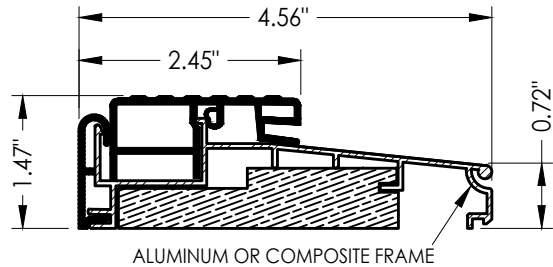
32 OUTSWING THRESHOLD WORLDWIDE
