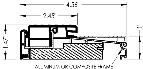
33 INSWING THRESHOLD w/ SIDELITE ADAPTER WORLDWIDE
