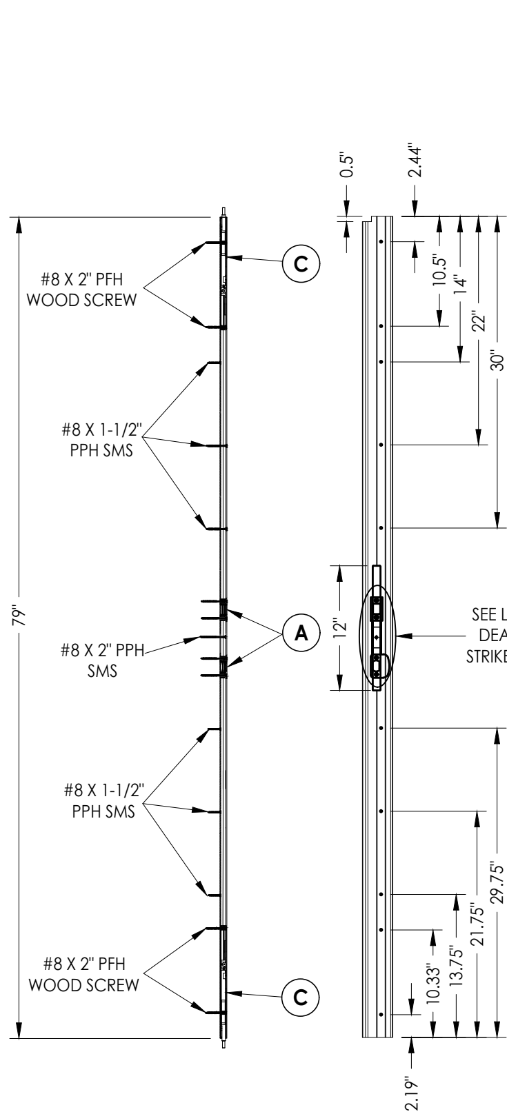
STANDARD ASTRAGAL ASSEMBLY
