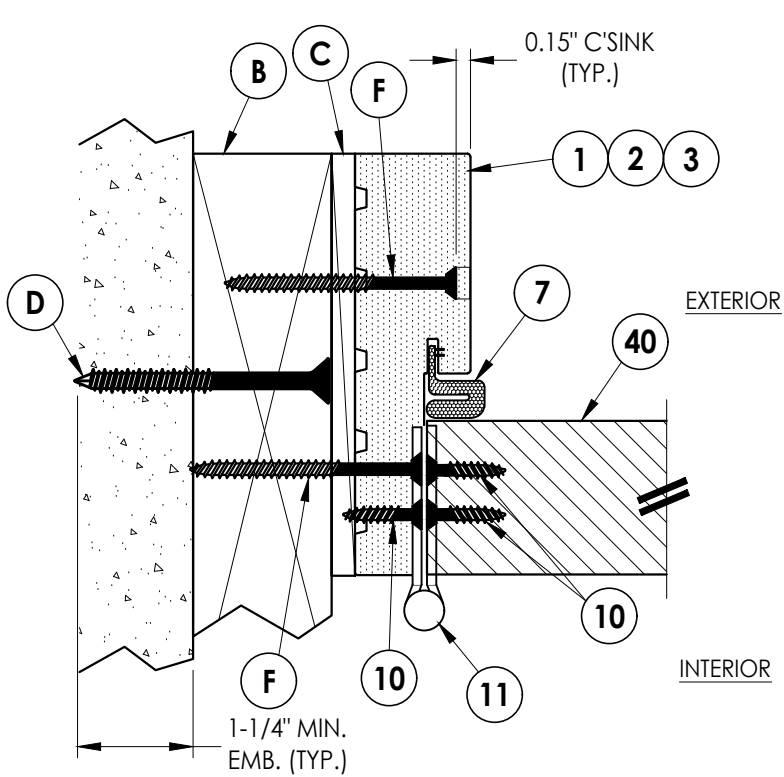
1 HORIZONTAL CROSS SECTION 5 Inswing Shown (Outswing Similar) 2X Buck Construction
