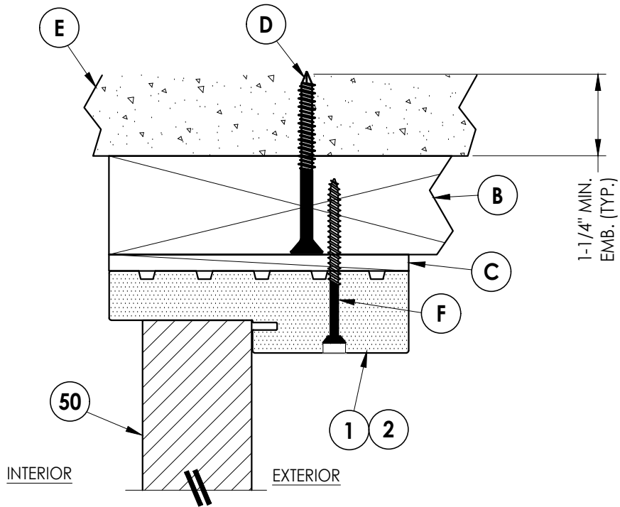
4 VERTICAL CROSS SECTION 5 Inswing Shown (Outswing Similar) 2X Buck Construction
