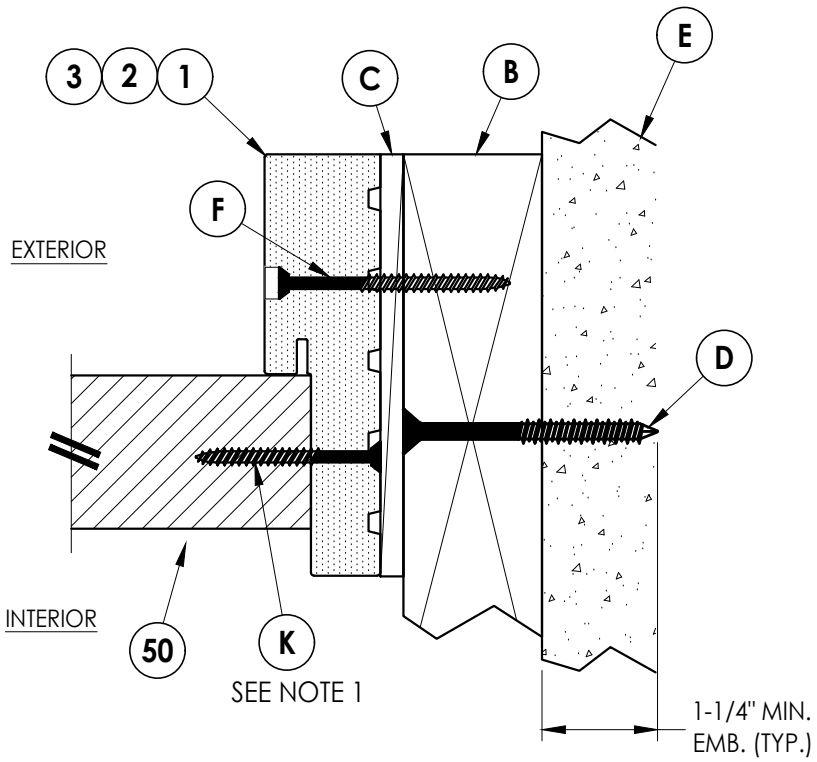
2 HORIZONTAL CROSS SECTION 5 Inswing Shown (Outswing Similar) 2X Buck Construction
