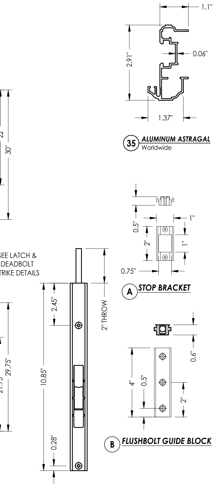
SLIDE LOCK FLUSHBOLT ASSEMBLY STANDARD ASTRAGAL
